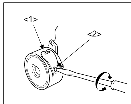
<1>: Bobbin case
