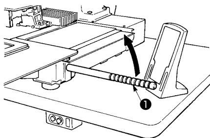
Maintenance position of the sewing machine
